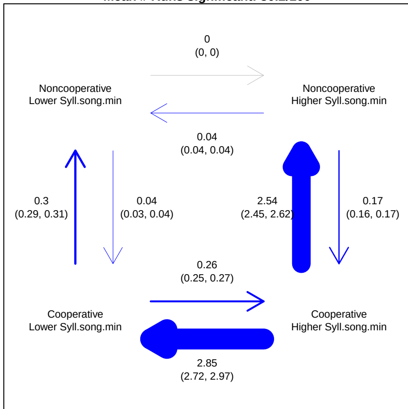
Thresholds \geq 9 - < 100 (18) Mean # Runs significant: 30.2/100
