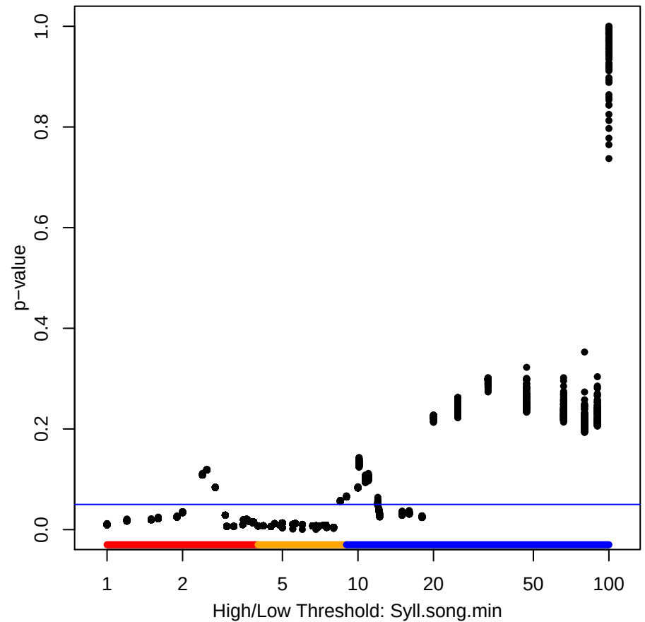
CoopBreed Syll.song.min Original threshold range: 1 - 100 (54)
