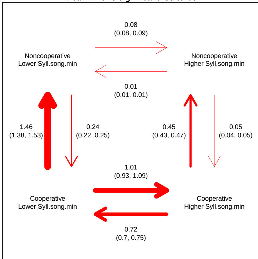
Thresholds \geq 1 - < 4 (18) Mean # Runs significant: 83.3/100
