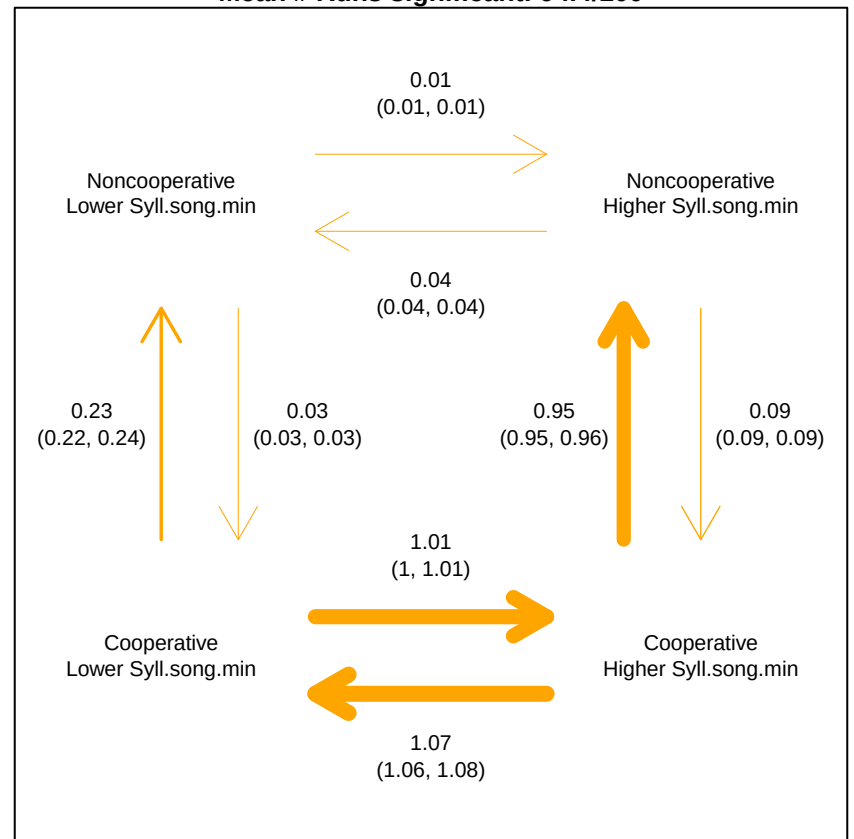
Thresholds \geq 4 - < 9 (18) Mean # Runs significant: 94.4/100
